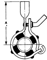
A24FCF Tubing Hanger (w/ 3/8" - 18NPT thread)
