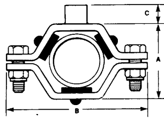
C24T Tubing Hanger (w/ 3/8" - 18NPT thread)
